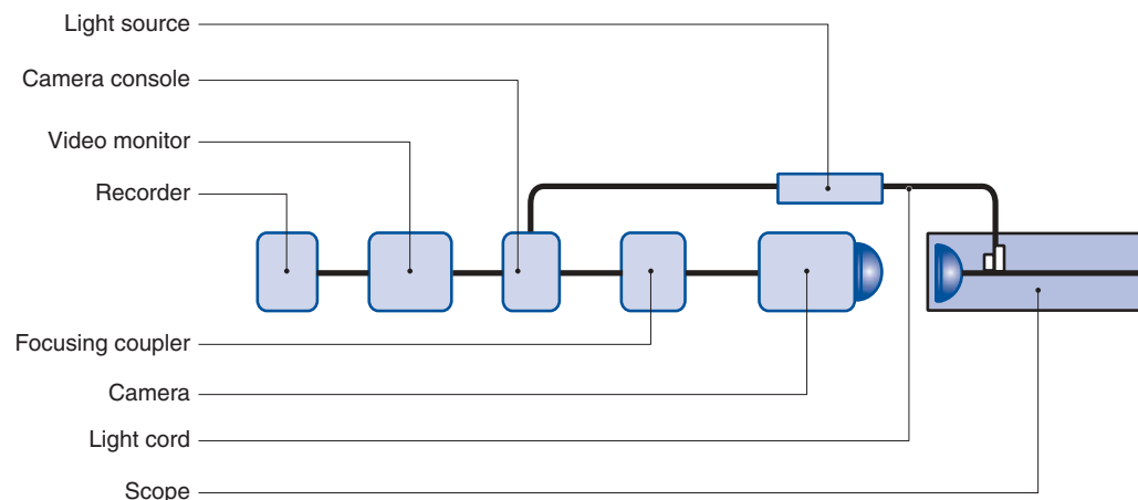
FIGURE 49-5 Schematic of equipment hook-up sequence.
