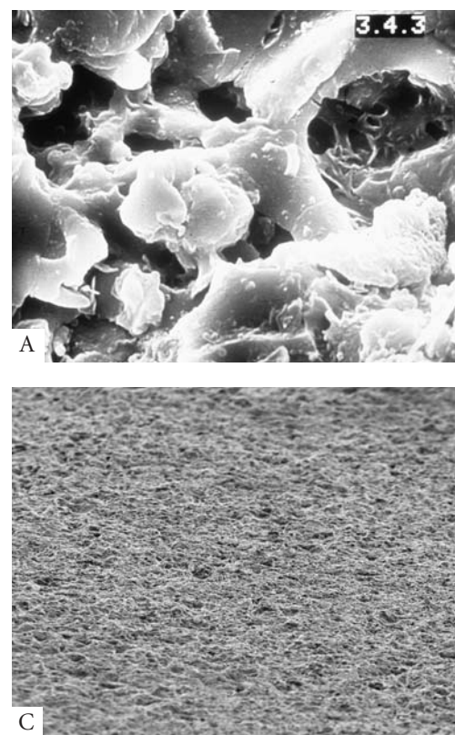
FIGURE 10-2 A, Titanium plasma-sprayed surface at high magnification. B, Acid-etched titanium surface at low magnification. C, Hydroxylapatite-coated surface at low magnification.
