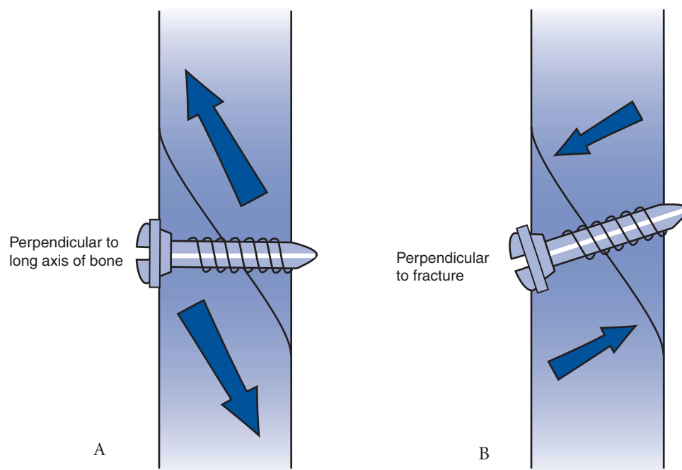
FIGURE 20-15 Improper (A) and proper (B) methods of placing lag screws. The screw should always be drilled perpendicular to the line of fracture to prevent sliding of the fragments during tightening of the screws.
