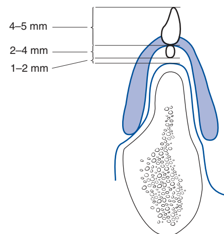
FIGURE 14-37 Minimum clearances needed for a bar-attached overdenture.
