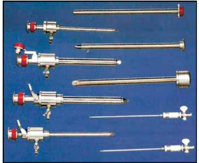
Fig. 49.5: Trocar and Cannula/verres needle
